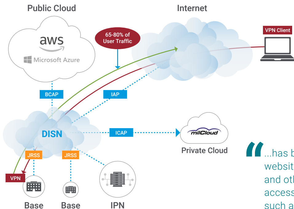
Figure 1 - Legacy VPN internet traffic flow.
